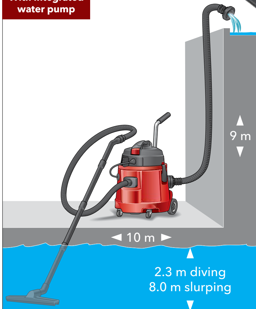
10 m dirty water hose with C-pipe connection
